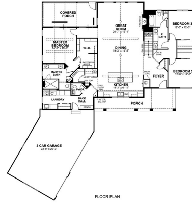
The Harper - Canted Garage Layout
